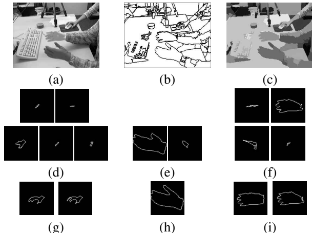
Figure 4. HCI dataset results. Candidate groups of regions generated for some frames. Notice there are 3 hands in the frame. (a) Original frame; (b) segmented image(boundary); (c) segmented image; (d) primitives around the third hand; (e) primitives around left hand; (f) primitives around the right hand; (g) the candidate groups for the third hand; (h) the candidate groups for the left hand; (i) the candidate groups for the right hand.
