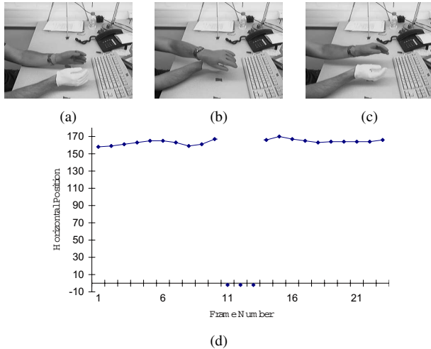
Figure 9. Ability to handle occlusions. Three frames from the “Rotate Down” gesture is shown in (a), (b), and (c). The estimated horizontal position of the hand is shown in (d). Note that there are no estimates for the frames for which there was occlusion, which shows that the best group was chosen correctly even across occlusions.
