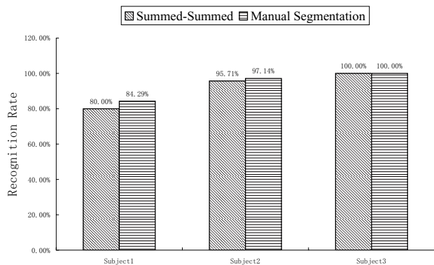
Figure 7. Recognition performance of each subjects separately, using Summed-Summed approach and Manual Segmentation.
