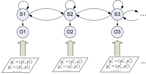
Figure 1. In frag-HMM, we do not have an unique observation sequence to match, rather we have a collection of possible observation sequences, implied by the sequence of multiple observations at each frame.
