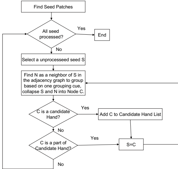
Figure 2. Flow chart of the grouping process used to generate each grouping layer.
