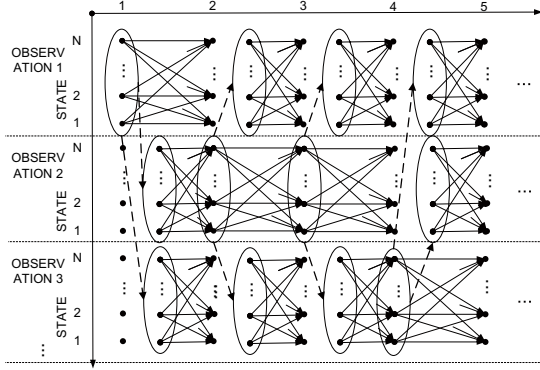
Figure 3. An illustration of the indexed forward process, the horizontal line represent the time, the vertical line correspond to the candidate observations and the sub-vertical line denotes the N states. Note at each time step, only one best observation is selected based on the previous selected observations and the forwarding results. In this example, the optimally selected observations (circled ones) are \langle 1, 2, 2, 3 \rangle .
