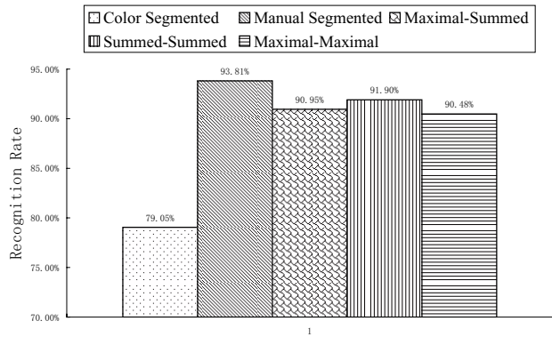
Figure 5. Recognition performance of 210 instances of 7 hand gestures for five different approaches. The first two are based on manual and color based segmentation of the hands. The next three does not use the knowledge of the hand color and take into account fragmented observations. The three corresponds to the three different kinds of probabilities that can be computed, P_{max,sum} , P_{sum,sum} , and P_{max,max} using the frag-HMM proposed in this paper.
