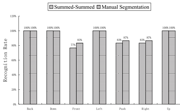
Figure 6. Recognition performance of each hand gestures, using Summed-Summed approach and Manual Segmentation.
